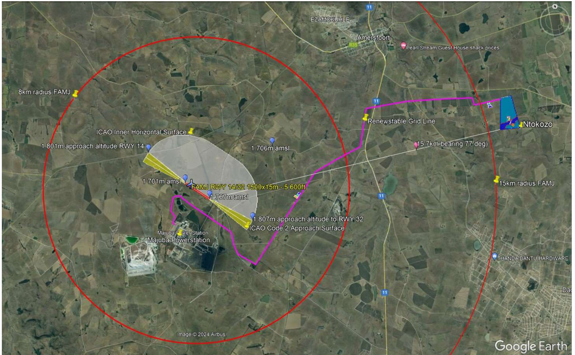
Figure 14: Approach Surfaces to FAMJ RWY14/32 with key distances & bearings to Ntokozo Solar Array
