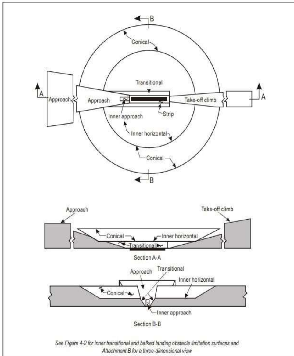
Figure 3: ICAO Obstacle Limitation Surfaces
