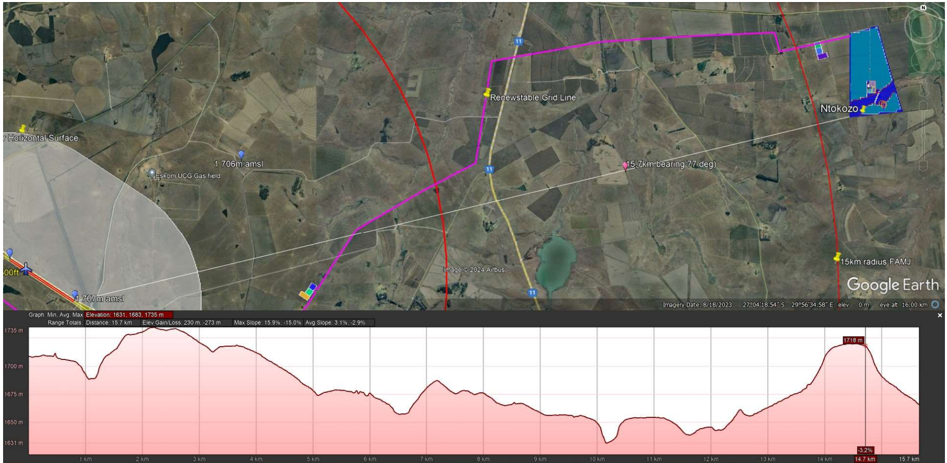
Figure 7: Elevation Profile from Extended Runway Centreline across Ntokozo Site
